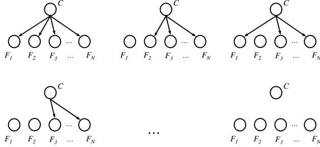
Figure 2: Enumerating all the 2^N possible naïve Bayes net structures.
