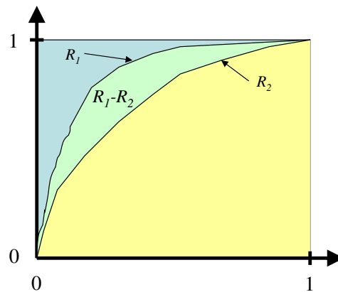
Figure 3: The performance metric \delta used in our experiments measures the fraction of ROC area captured by our classifier (with ROC area R_1 ) versus some other classifier (with ROC area R_2 ).
